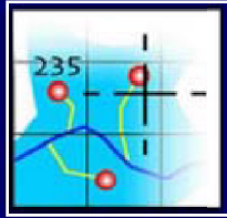
AddressIt 2.2
